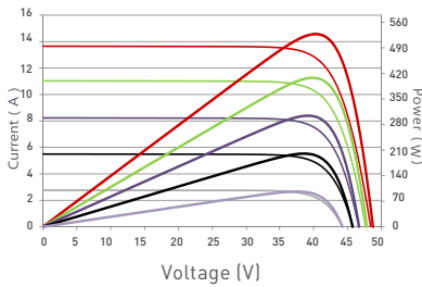
Current-Voltage & Power-Voltage Curves (535W)
