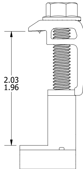
ASSEMBLY CHECK
