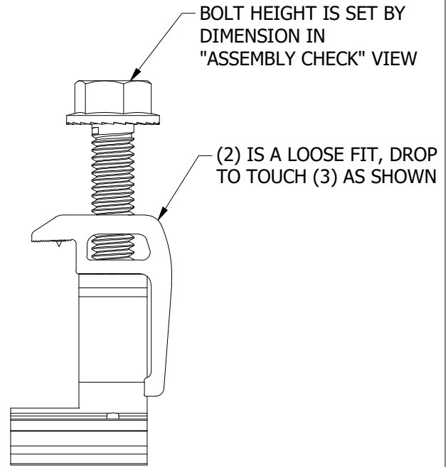
AS SHIPPED
